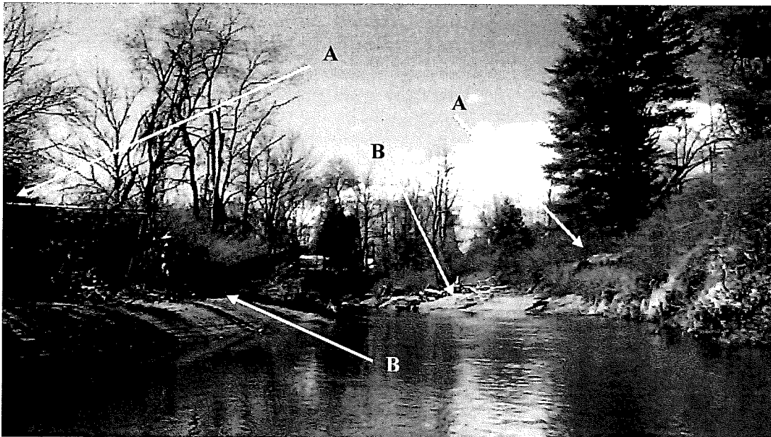
Figure 1 Embryonic active floodplain developing in incised channel. Stage IV of channel evolution.
